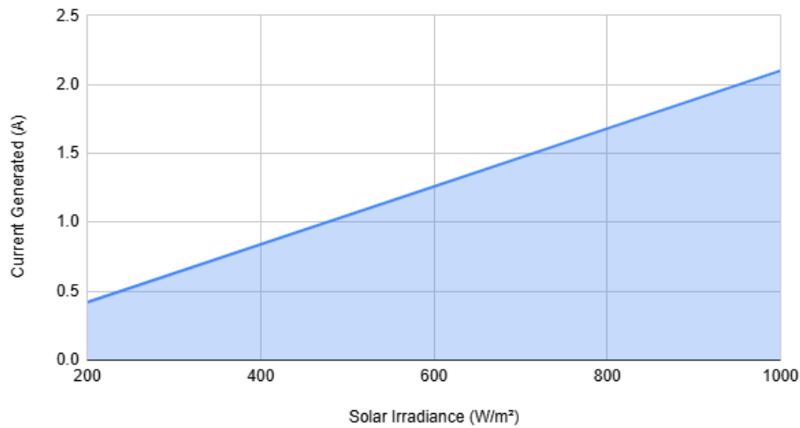
Current generation of 15W solar panel under different sunlight intensities
